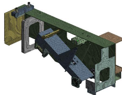
Fine meshing attributes are applied to the combination of mid-plane surfaces and solid components
